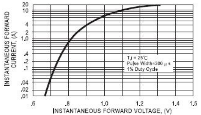
FIG. 2 - TYPICAL INSTANTANEOUS FORWARD CHARACTERISTICS
