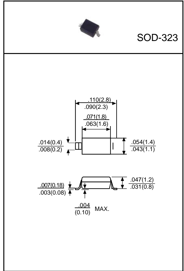
Dimensions in inches(millimeters)
