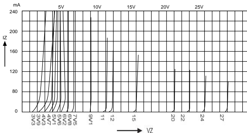
Breakdown characteristics DL47-SERIES
